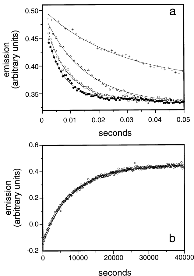
FIGURE 2: (a) Time course of emission after mixing of 0.4 \mu\text{M} Pep-1F and 2, 4, 8, \Delta , 10, \bullet \mu\text{M} S-protein at 10 °C in 10 mM MOPS, pH 6.7, in a stopped-flow device. The sample was excited at 496 nm, and emission at all wavelengths was monitored at 90°. The data are fitted by single-exponential curves (solid lines). The pseudo-first-order rate constants from the fits are defined as k_{\text{obs}} with units of \text{s}^{-1} . (b) Time course of emission after mixing 0.2 \mu\text{M} of the complex between Pep-1F and S-protein with 200 \mu\text{M} unlabeled Pep-1. The other conditions are identical to (a). The sample is excited at 496 nm, and emission at 520 nm is monitored. The time course is fitted by a single-exponential curve (solid line). The observed first-order rate constant of (1.19 \pm 0.08) \times 10^{-4} \text{ s}^{-1} is k_{\text{off}} , the dissociation rate constant for the complex.
