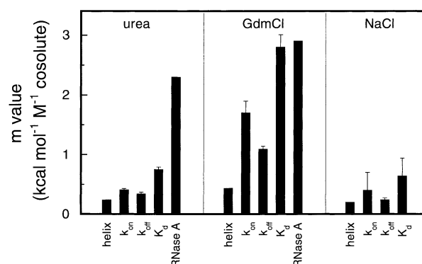
FIGURE 9: Effects ( m -values) of urea, GdmCl, and NaCl on k_{\text{on}} , k_{\text{off}} , and K_d ( k_{\text{off}}/k_{\text{on}} ) for the Pep-1F/S-protein complex (Table 2). The data are compared to the m -value for the unfolding of RNase A from Pace and co-workers (34), and the m -value for unfolding a 10 residue alanine-based helix calculated from the parameters of Smith and Scholtz (37).
