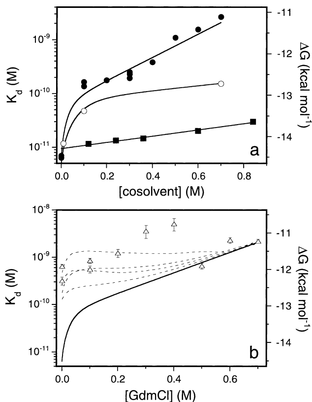
FIGURE 6: Apparent dissociation constant ( K_d , left axis, \Delta G = -RT \ln K_d , right axis, T = 283 K) for the RNaseS* complex (Pep-1F) as a function of cosolvent concentration. The conditions are as described in Figure 2 except for the presence of cosolvent. (a) The kinetically determined values of K_d ( =k_{\text{off}}/k_{\text{on}} ) are shown in the presence of (●) GdmCl, (■) urea, and (○) NaCl. The standard errors are approximately the size of the data points. The solid lines through the data are calculated from eq 5 using the parameters in Table 2 as described in the text. (b) The apparent value of K_d measured by the equilibrium titration method, \Delta , as a function of the GdmCl concentration. The solid line is the dissociation constant calculated from kinetic data, as described in (a), and is shown for comparison. The dashed lines are drawn through K_d values from simulated equilibrium titrations in which Pep-1F is supposed to contain 5% or 10% of a weakly binding contaminant, as described in the text.
