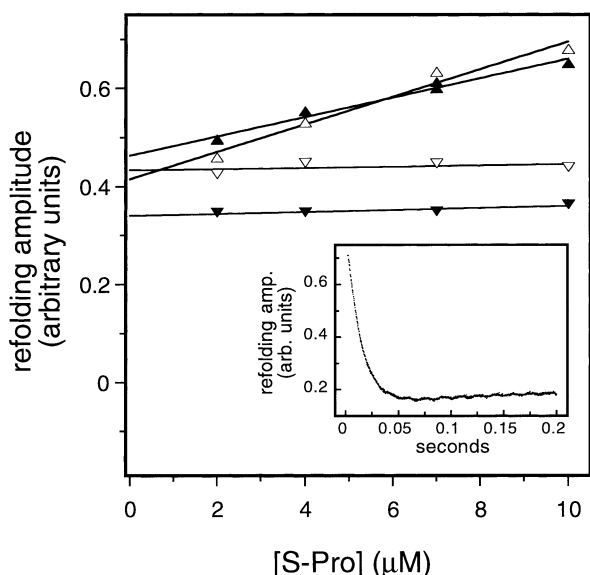
FIGURE 4: Amplitudes for the association reactions of M13A-1F and S-protein as a function of the concentration of S-protein at ( \Delta ) 1.7^\circ\text{C} ; ( \blacktriangle ) 9.7^\circ\text{C} , ( \blacktriangledown ) 19.3^\circ\text{C} , and ( \nabla ) 29.0^\circ\text{C} . The conditions are as described in Figure 2a except for the variation in temperature. Inset: refolding time course for M13A-1F and 10 \mu\text{M} S-protein at 1.7^\circ\text{C} showing the second, slower increasing phase.
